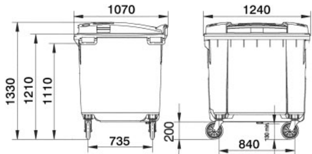
nominal dimensions
